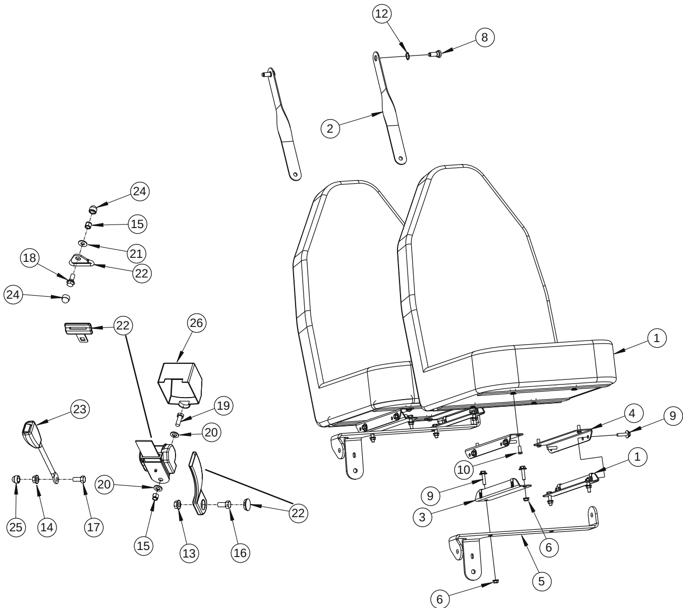
ASSY, BUCKET SEAT RIGHT - FIXED - SEE NEXT PAGE FOR PARTS LISTING
